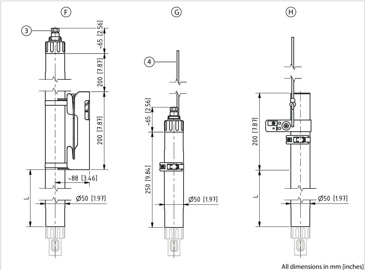
All dimensions in mm [inches]
